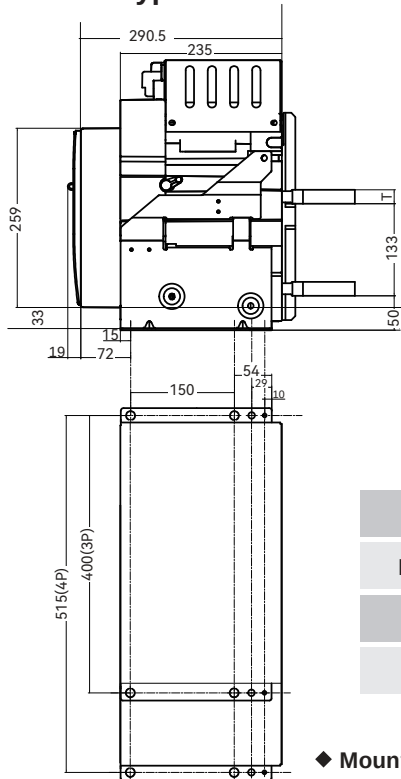
MGW6-4000 ACB Fixed type(3P,4P)
