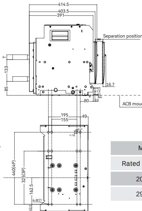
◆ Mounting dimensions
