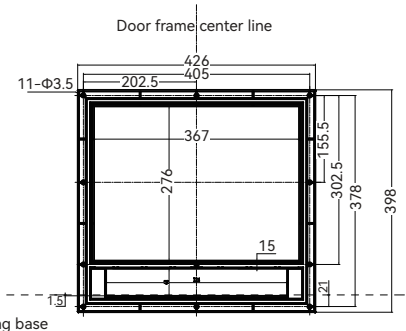
◆ Mounting hole pitch
