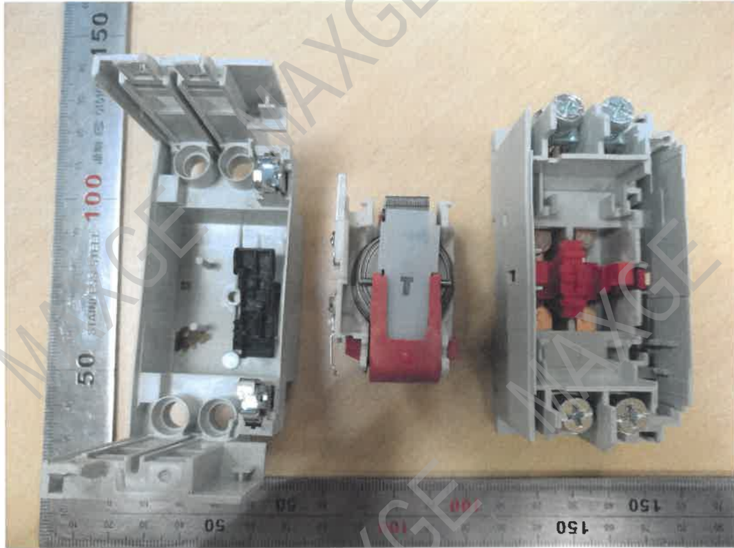
Inner construction of 4P, 63A
